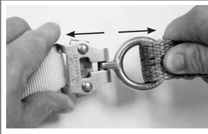
Figure 12 – Failed Connection
