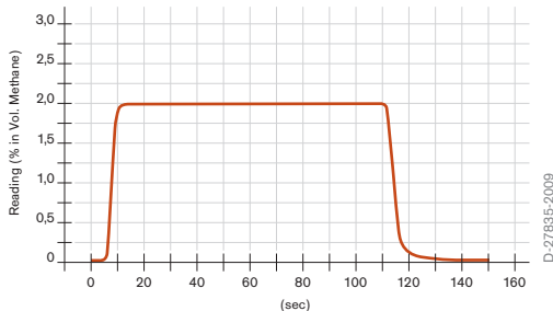
Response time of DrägerSensor CatEx 125 Mining PR in X-am 5000
