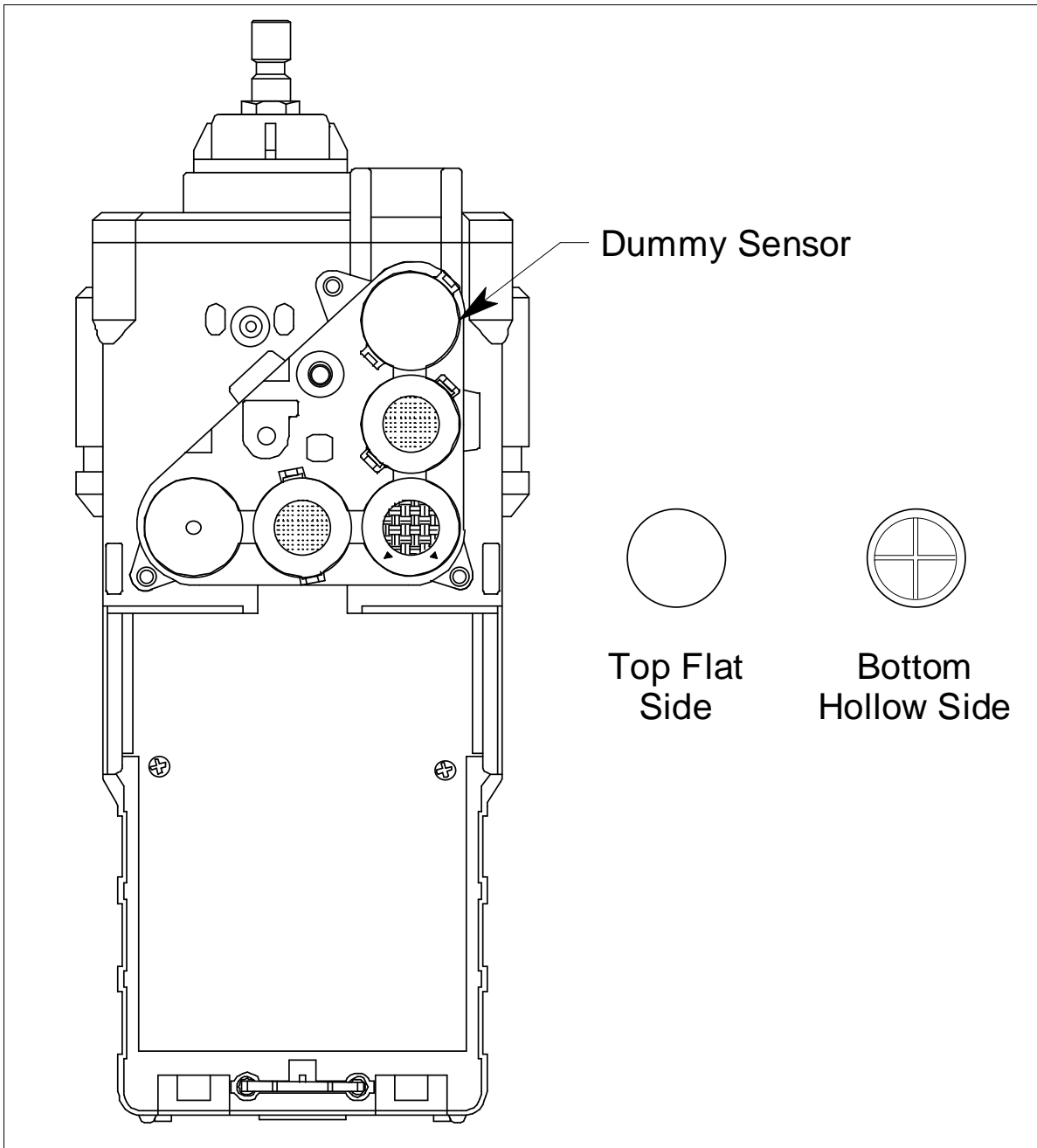
Figure 3: Dummy Sensors
