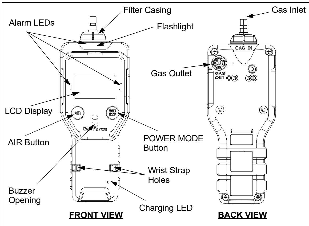
Figure 1: Component Location
